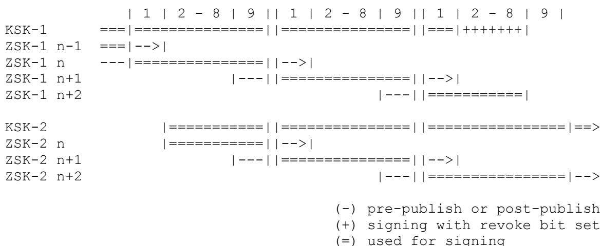
Figure 3: Diagram of a 270-day span with concurrent KSK and ZSK rollovers with differing algorithms
