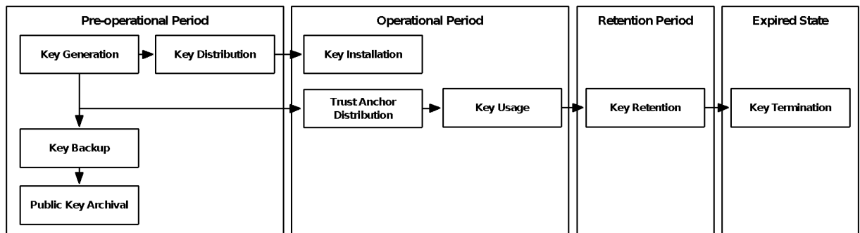
Figure 1: Key lifecycle for KSK
